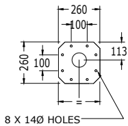
MOUNTING BASE PATTERN
